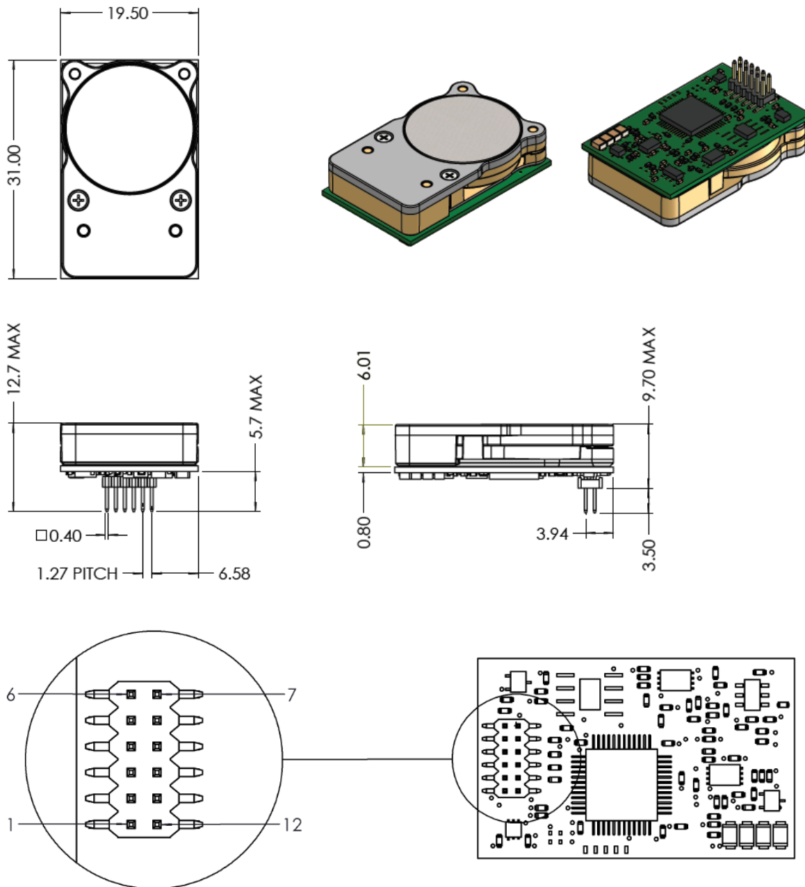
Bottom View
